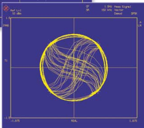
Vector diagram of distorted modulation signal
